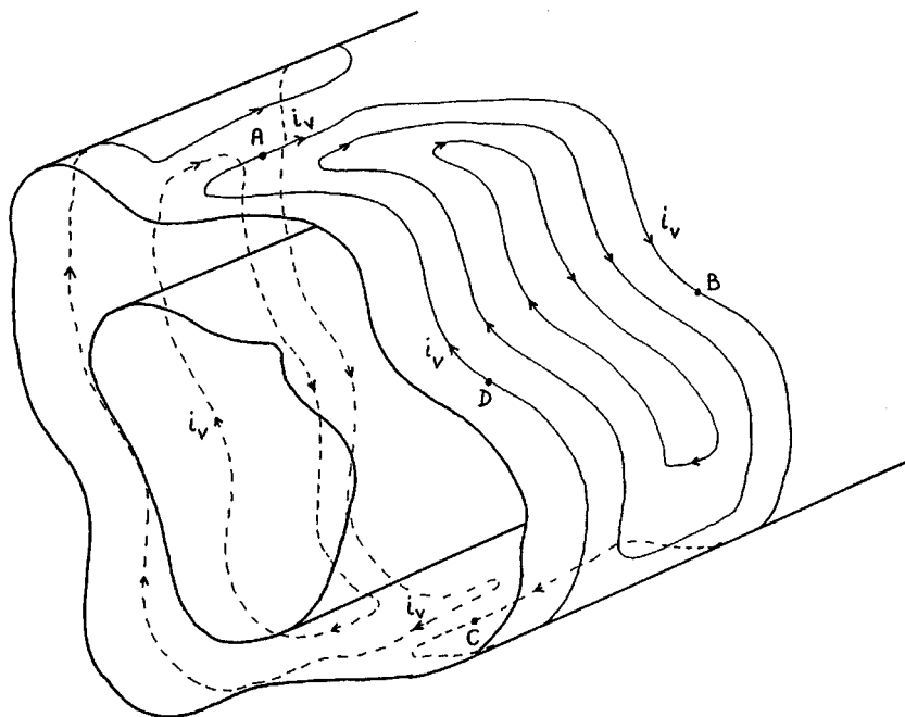
Fig. 2. A combination of j_{VO1} per-unit-length current and i_{VA1} current.
